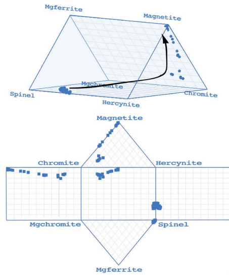
Fig. 12. Plotting the end-members of the spinel group mineral from ophiolites on the Magnetite prism to verify the compositional trend detected using a 2D scatterplot.
