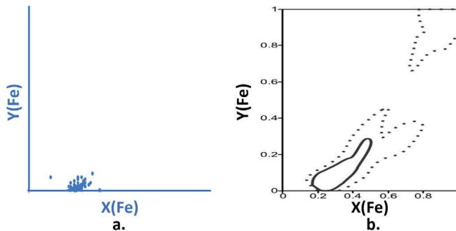
Fig. 8. Matching rectangular faces of the prism a. with the compositional field for lithospheric mantle xenoliths b. delimited contour lines based on Barnes and Roeder [1].
