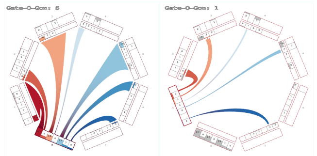
Figure 7: Two Gate-O-Gons of the same analysis session, illustrating how movements between gates can differ. Left: Gate-O-Gon of the start area, a lot of animals returned from most higher gates, visible from the thick straps. Right: Gate-O-Gon of gate 1, where only a few animals returned to in relation to the start gate.
