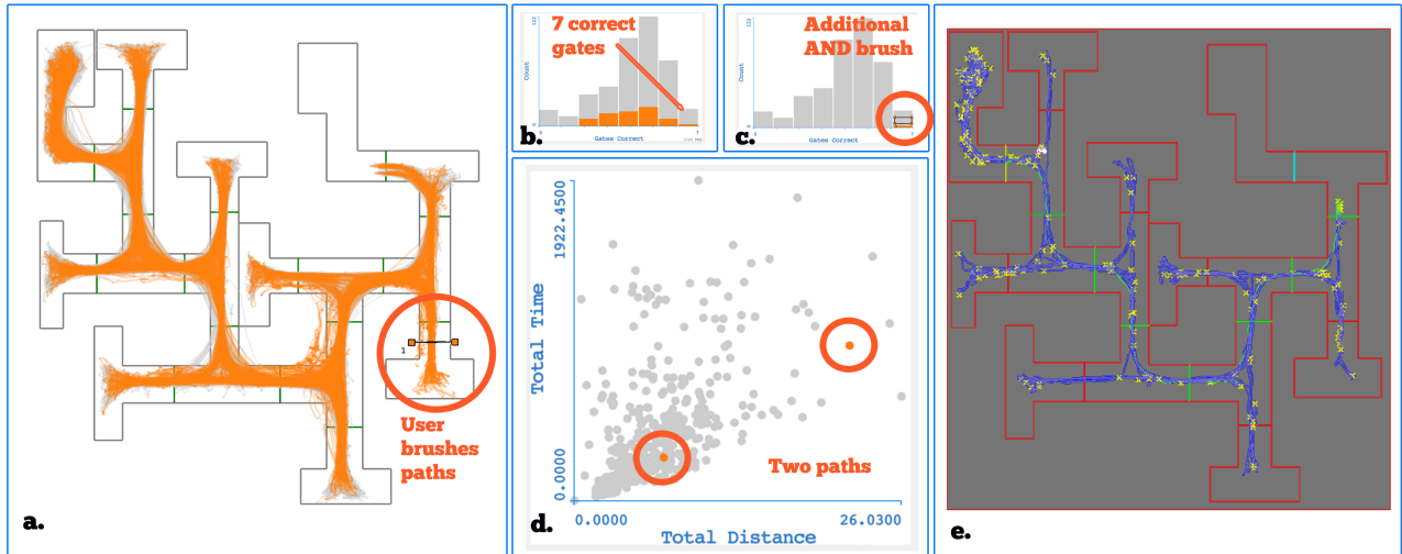
Figure 8: A possible analysis session for the \approx 400 trajectory ensemble data, using the T-Maze Explorer. a) shows all the trajectories of the dataset superimposed on the Multiple T-Maze. A brush was used to select all trajectories where animals went into the dead end corridor of gate 7. b) A histogram showing the distribution of correct decisions, before brushing. c) The histogram from b) after a brush to 7 correct gates was applied. It now highlights the remaining trajectory data. d) A scatter plot showing the correlation between Total Time and Total Distance. Only two data points meeting the brushed criteria are highlighted. e) Single Trajectory View static depiction of speed. Yellow markers indicate the animals position every 5 seconds. Here the trajectory with higher total time and distance from the two brushed trajectories was selected. The animal made the correct first choice for each gate but ventured back to previous gate segments quite often.
