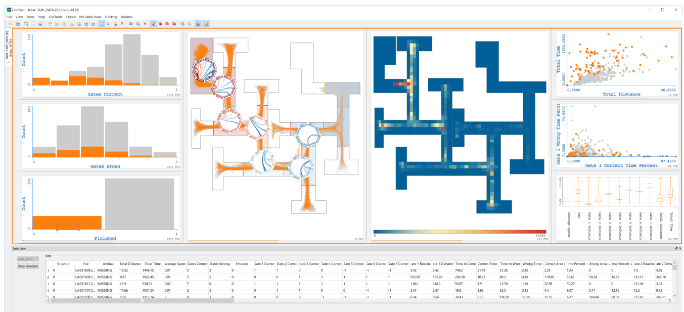
Figure 1: The T-Maze Explorer – the proposed system for Multiple T-Maze data exploration. The user can combine different interactive views, here t-maze specific views are shown in the middle. In this instance diverse charts – left and right views – give an overview of single or multiple scalar features of animal trajectories as well as detailed descriptive statistics – table in the bottom. All views are linked.
