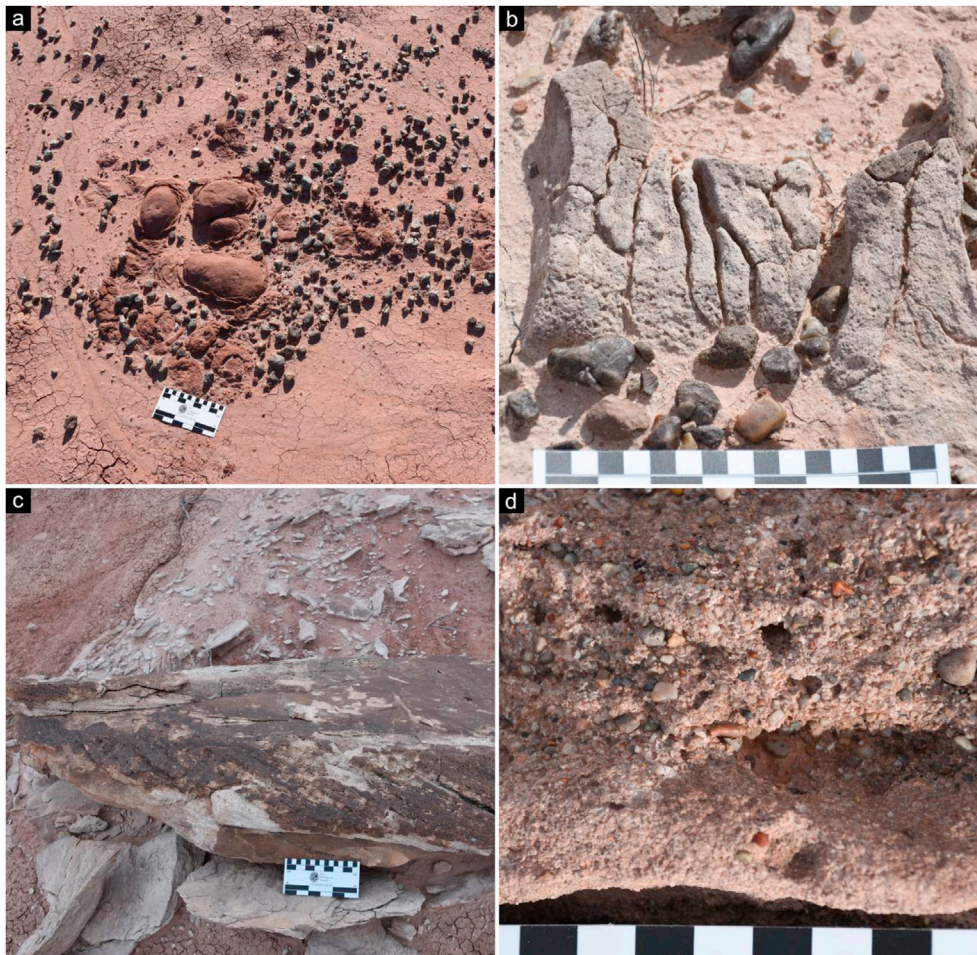
Fig. 3. Characteristic sedimentary facies encountered during field reconnaissance of the MURFI study area. a) Numerous small outcrops of silty to very fine sand (red/purple in color) were common, particularly in areas of reddish soil. b) Fine-to medium-grained quartz-rich sandstone found cropping out from lighter colored soil. Both the red silt-to-very fine sand and white fine-medium sands were highly fractured and showed onion skin weathering or cracked textures. The white sands were often trough cross laminated, and found in isolated, elongated exposures which could be interpreted as barforms, fining to the northwest. c) Cross-bedded pebbly conglomerate from the upper platform of 'Big Mesa' – an inverted fluvial channel section in the MURFI study area. d) Texture of the pebbly conglomerate in c) showing the very poor sorting and polymictic composition, with sub-rounded to sub-angular clasts within a quartz-rich matrix. The smallest black and white divisions of the scale bar are 1 cm in each photograph. Image credit: Robert Barnes and Steven Banham. (For interpretation of the references to color in this figure legend, the reader is referred to the Web version of this article.)
