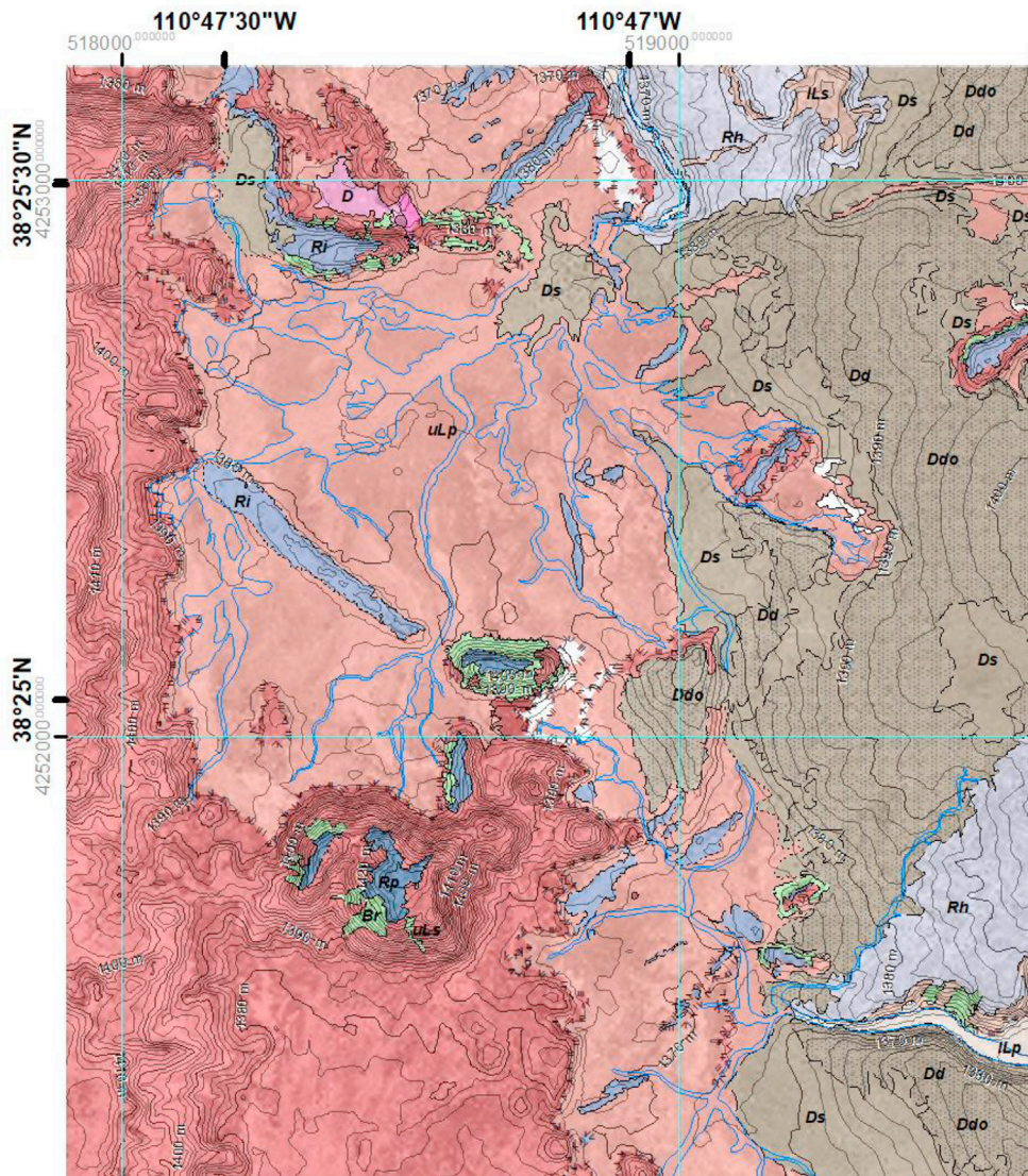
Fig. 10. Subset of the photogeological map of the landing site region. Reds = Layered (scarp and plains-forming) Formations, Blues = Resistant Formation, Browns = Dark Formation, Green = out-of-situ rubbly boulder and debris, White = Anomalously Bright Unit (a distinctive unit in the Layered Formations). Blue lines = modern alluvial deposits and green lines = targets. Additionally Pinks indicate anthropogenic features, such as a dam structure in the north of the region. Graticule and grid show WGS1984 and UTM zone 12N; pale blue gridlines are 1 km apart. (For interpretation of the references to color in this figure legend, the reader is referred to the Web version of this article.)
