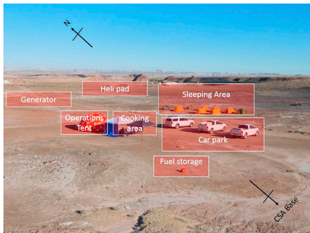
Fig. 4. MURFI basecamp showing key locations. Image credit: Mike Curtis-Rouse.
