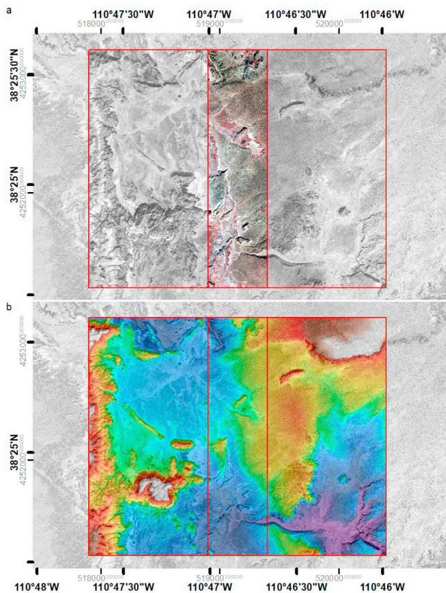
Fig. 9. The MURFI field site area mapped using Mars-like remote sensing data (cf. black box showing study area in Fig. 2b). An area ~2 by 3 km was mapped. a) A simulated HiRISE image (Worldview 2), including the central color strip and the lateral greyscale areas. b) 5 m resolution DTM showing topography. Note that this DTM actually has lower resolution than the best Mars DTM data (5 m/pixel vs 1 m/pixel). Graticule and grid show WGS (World Geodetic System) 1984 latitude and longitude and UTM (Universal Transverse Mercator) zone 12N projection scale information. Image credits: see Table 5. (For interpretation of the references to color in this figure legend, the reader is referred to the Web version of this article.)
