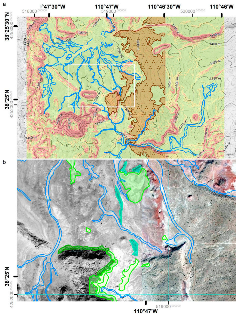
Fig. 12. Hazard and science target mapping. a) Hazards within the wider mapping region. Modern Alluvial hazards are outlined in blue. In the background, slopes <5^\circ are colored green, slope 5^\circ - 10^\circ are yellow, slopes of 10-15^\circ are orange, and slopes >15^\circ are red. The brown area is the 'Dark Dappled Unit', Ddu – interpreted to be densely covered with boulders and vegetation. White box shows position of Fig. 12b b) Possible science targets in the central portion of the remote sensing map region. Dark greens show Resistant Formation outcrops or float rocks that could be rover accessible, mid-green are other possible bedrock outcrops, and bright green show the edges of the Layered Plains Unit or the Anomalously Bright Unit (Abu). The blue lines show modern alluvial hazards. Background image is a HiRISE-like image (Worldview 2). Graticule and grid show WGS1984 and UTM zone 12N. Image credits: see Table 5. (For interpretation of the references to color in this figure legend, the reader is referred to the Web version of this article.)
