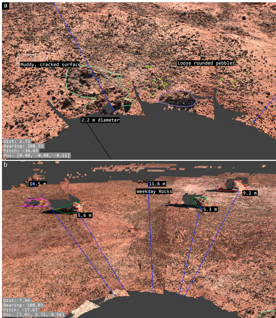
Fig. 8. PRO3D example outputs. a) Near-field view showing annotations made onto the PRO3D scene. b) Distance measurements, useful for drive planning, made using PRO3D – in this case, to the ‘weekday rocks’ using sol 1 data.
