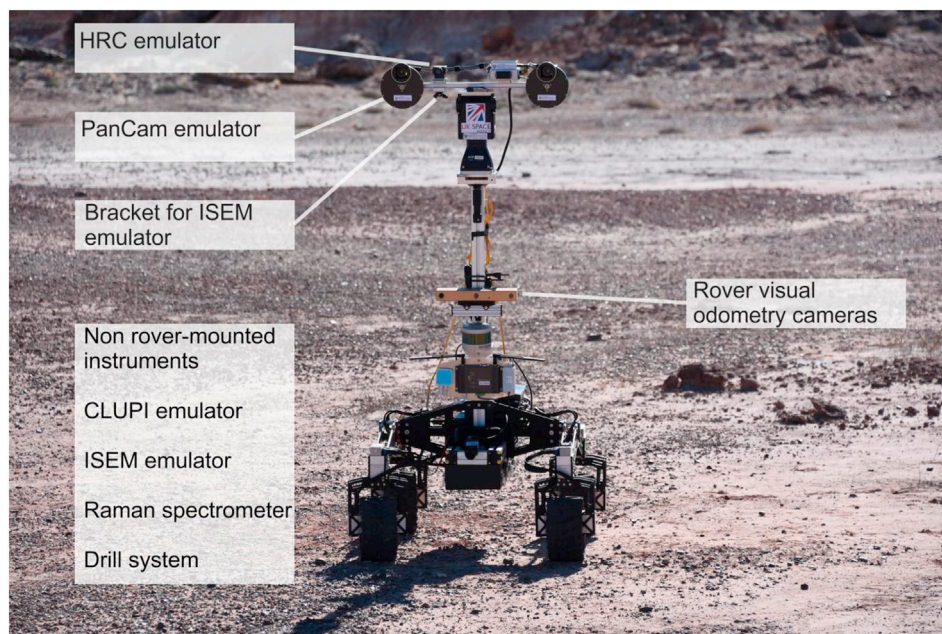
Fig. 6. The MURFI rover platform showing the rover instruments. The main imaging instruments were rover-mounted, but the spectrometers were mainly used demounted from the rover for the convenience of the field team. The ISEM emulator could be used mounted or demounted. See Fig. 1 for scale. Image credit: Mike Curtis-Rouse.
