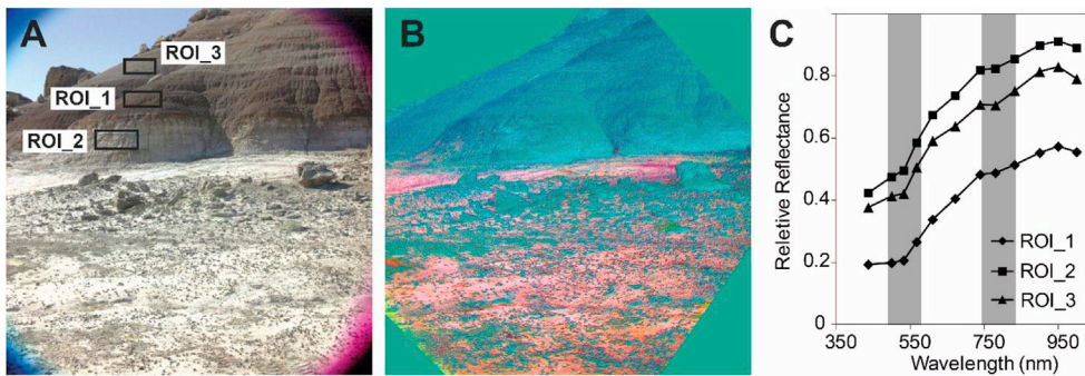
Fig. 19. WAC Multispectral results. a) Enhanced color AUPE WAC image of Big Mesa showing location of Region of Interest (ROI) targets. b) Principal Component Analysis (PCA) false-color Left-WAC AUPE image using RGB filters, revealing Big Mesa to comprise spectrally-similar material. c) AUPE spectra extracted from the three ROI targets, all with a strong absorption at 530 nm and a weak absorption at \sim 800 nm. (For interpretation of the references to color in this figure legend, the reader is referred to the Web version of this article.)
