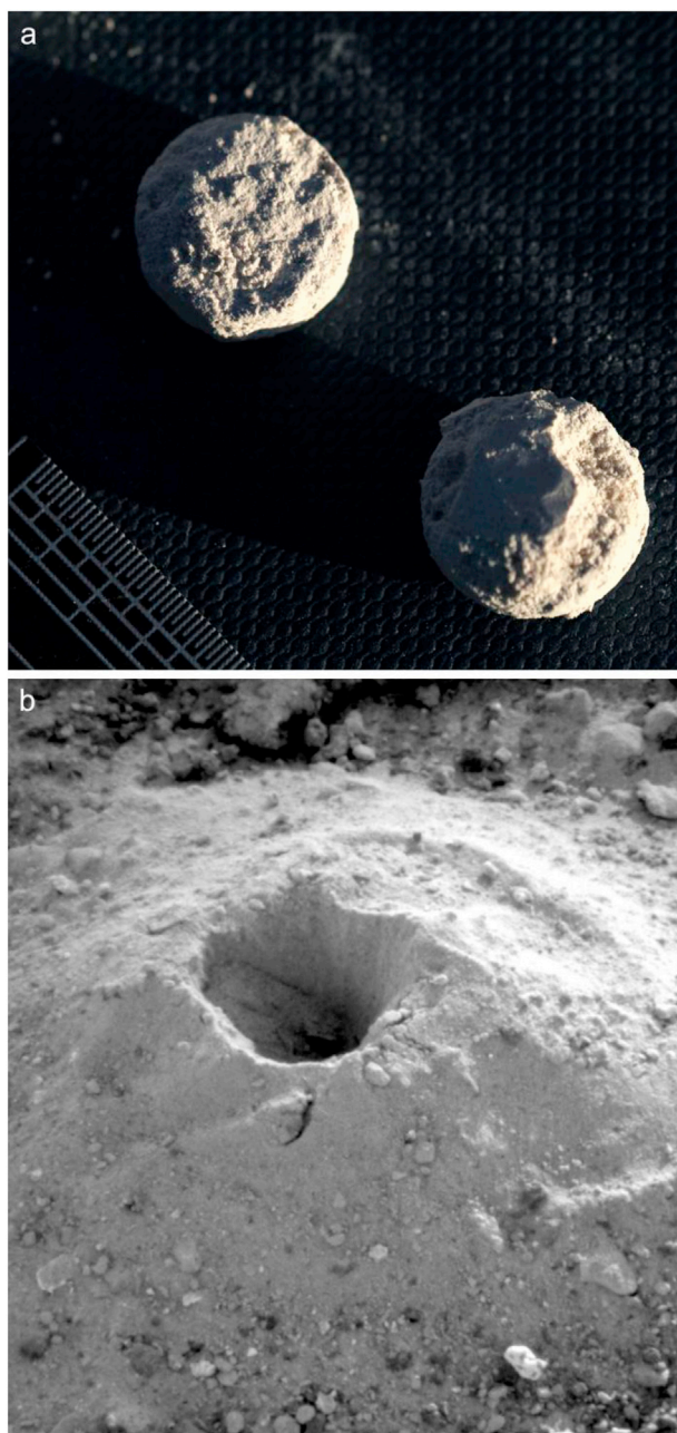
Fig. 16. Results of drilling. a) Small parts of drill core obtained. Scale bar lower left is in mm. The CLUPI emulator image of the drill core pieces showed that they contained many fine sand-sized grains, and were not mudstone as had been predicted. b) The ‘drill tailings’ that resulted from the drilling. This debris pile was actually constructed by the field team to mimic a real drill-core debris cone as the majority of the depth of the excavation was made using a spade, not a deep drill-corer for reasons of field efficiency. Only the final few centimeters of the excavation was done with a corer. The debris material was obtained from the bottom of the excavation to provide a realistic material sample.
