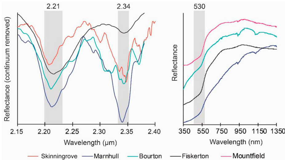
Fig. 20. ISEM emulator reflectance spectra in the short-wave infrared (left) and visible to near-infrared regions (right) for a variety of targets. Fiskerton is a ground-surface target of soils containing mud-cracks analyzed on sol 1; Marnhull is a small boulder set within soils, Mountfield an area of anomalously high albedo soils, and Bourton a large patch of high albedo material analyzed during the ‘drive-by’ analysis – all were analyzed on sol 2; Skinningrove is an area of ground containing the drill site, analyzed on sol7.
