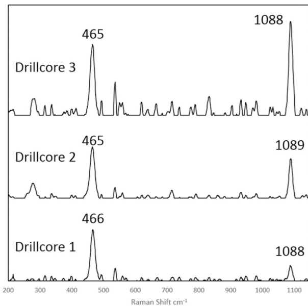
Fig. 21. Representative Raman spectra from the three drill core pellets. Spectra have background and fluorescence subtraction with all negative values set to 0. Wavenumber 466\text{ cm}^{-1} indicates quartz, will 1088/1089\text{ cm}^{-1} indicates calcite.
