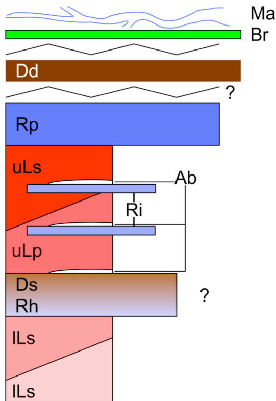
Fig. 11. Proposed stratigraphy based on remote sensing mapping. Zigzag lines indicate unconformities or poorly constrained contacts. Ma = Modern alluvial material. Br = Blocky rubble unit; Dd = Dark dappled unit (part of the Dark Formation), Rp = Resistant Plateau Unit (part of the Resistant Formation), uLs and uLp are upper Layered Formation Units (Scarp and Plains-forming respectively), Ab = Anomalous Bright Unit (part of Layered Formation), Ri = Resistant Interbedded Unit, Ds and Dh are part of the Dark Formation (Smooth and Hummocky respectively), ILs and ILp are Lower Layered Formation Units (Scarp and Plains-forming respectively).
