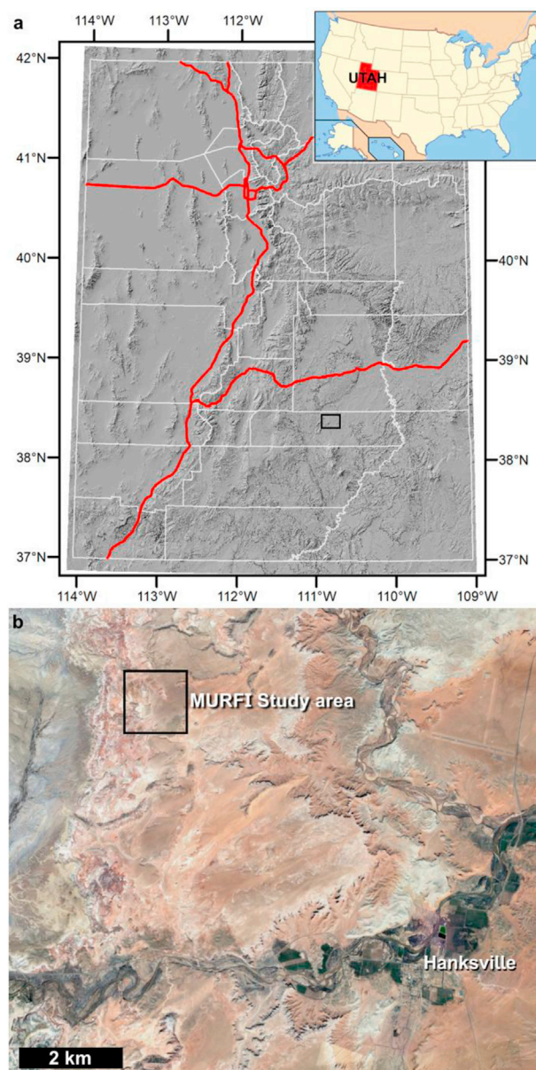
Fig. 2. Location of study area. a) Utah state map (above) showing major interstate roads (red) and county boundaries (white) overlain on a 100 m/pixel topographic hillshade map. The black box shows the location of the close-up view in (b). b) Close-up view showing MURFI study area as black box and location of nearest town (Hanksville). Image credit: Utah AGRC/GoogleEarth/Wikipedia. (For interpretation of the references to color in this figure legend, the reader is referred to the Web version of this article.)
