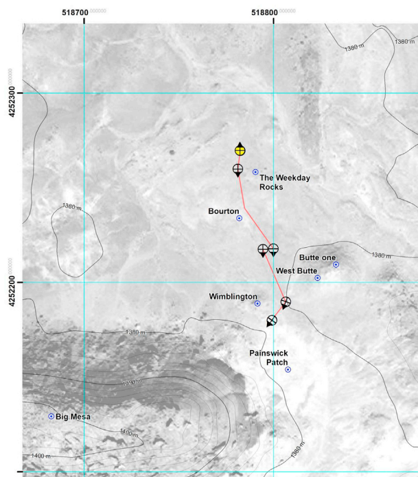
Fig. 13. Localization and drive calculations for the MURFI ExoMars rover-like mission, including some of the key targets and their locations. Note the Sol 5 localization recalculation that resulted in the rover positioning being moved ~5 m to the west. Graticule and grid show UTM zone 12N so blue lines are 100 m apart. Dark lines are 2 m contours based on the 5 m DTM. Image credits: see Table 5. (For interpretation of the references to color in this figure legend, the reader is referred to the Web version of this article.)
