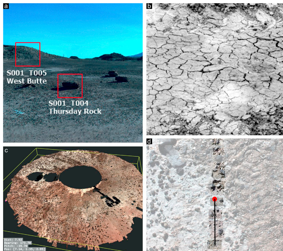
Fig. 15. Target examples. a) Sol 1 targeting example showing HRC field of views and target names and codes superposed on a portion of the sol 0 color panorama. b) The sol 2 HRC ‘drive-by’ image of the Bourton area – this image showed that Bourton was surficial materials and not bedrock. c) PRo3D scene of the local workspace near the rover as the SWT prepared to select the final drill site. PRo3D allowed size and distance to be measured accurately. The two dark circles to the left of the image were vegetation. d) Images from the ‘CLUPI Ladder’ superposed on a plan view, re-projected WAC color image. The red circles shows the chosen drill target location and the black line the drive distance required to reach that point. (For interpretation of the references to color in this figure legend, the reader is referred to the Web version of this article.)
