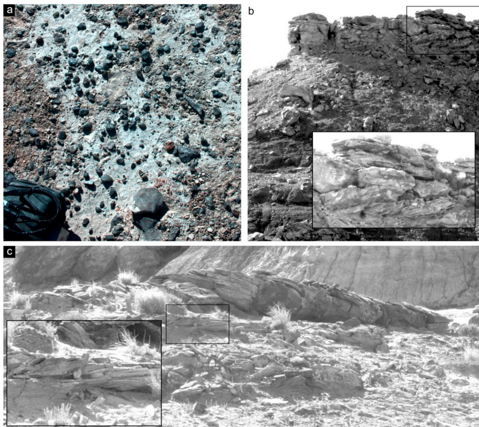
Fig. 17. Example science observations and interpretations. a) AUPE image of float rocks and surface texture. Note rover wheel for scale. b) HRC image of resistant material on top of Big Mesa. Layering can be seen, as well as probable crossbedding (inset). This material was therefore interpreted to be a sandstone. c) HRC image mosaic showing more possible cross-bedding (inset) in the 'Wimblington' target area. The SWT were not convinced this outcrop was in-situ, however.
