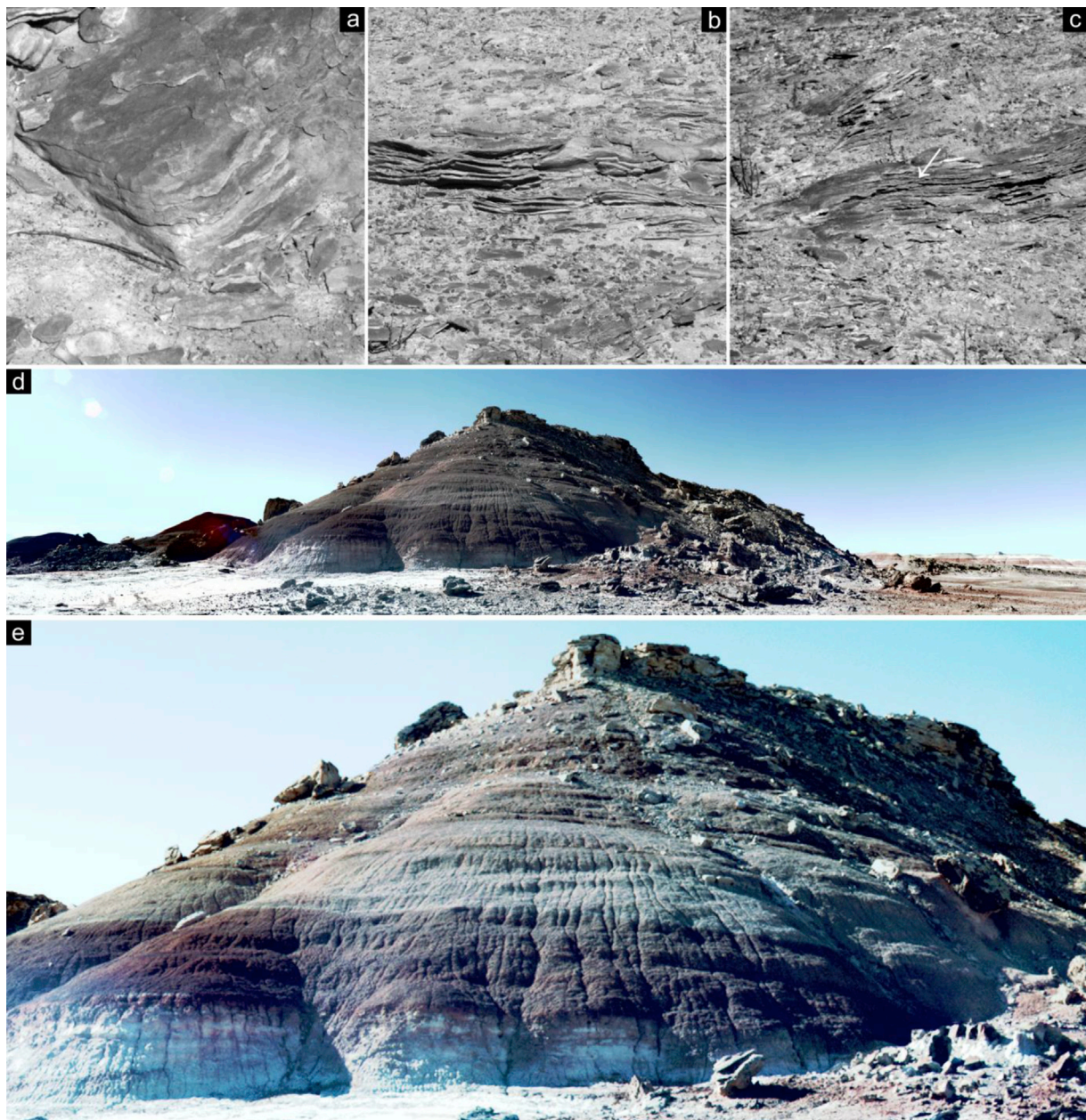
Fig. 18. Examples of science outcomes. a) HRC image of a portion of the ‘Cransford’ target, a layered outcrop of areas of soil overlying areas of apparently in-situ bedrock. The bedrock areas comprised 15–20 cm thick (based on PRO3d measurements) layered exposures, each composed of thickly laminated or finely bedded material interpreted to be sandstone. b) HRC image of another part of Cransford showing recessive interbeds. c) HRC image of a third area in Cransford, showing possible cross cutting, non-parallel bedding (arrowed), and possible subtly undulating bedding (right of arrow) d) WAC color mosaic of Big Mesa, showing the Resistant Formation (top, and materials shed to the sides) and the Layered Formation (lower part of outcrop, showing bands of whitish, brown and red material; interpreted to be much finer material), making up for the majority of the scene. At the far right of the scene are similarly colored layers in the distance. Note that sun-angle was consistently poor for imaging Big Mesa. e) Color-stretch close-up of the layering in Big Mesa, showing at least four different tonal-types, and highlighting the modern rill-forms that incise the outcrop. Big Mesa is ~22 m high. (For interpretation of the references to color in this figure legend, the reader is referred to the Web version of this article.)
